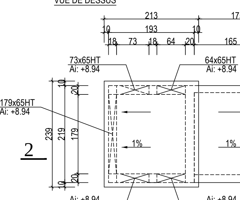
DETAIL "1" VENTILATIONS
